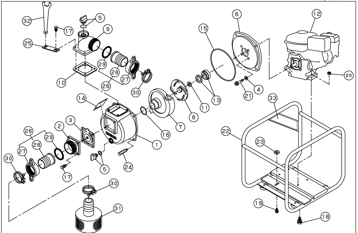
DWG No.012947701 MODELE:STV-100X FORM:STV-100X-BAE-0
